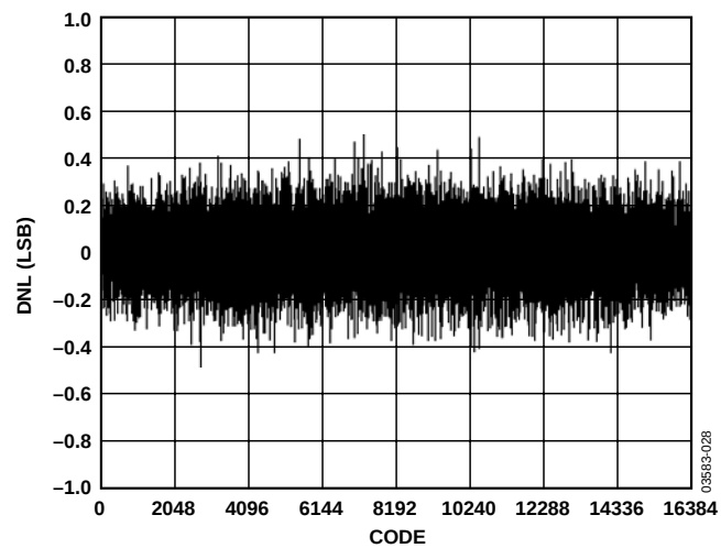
Figure 19. Typical DNL
