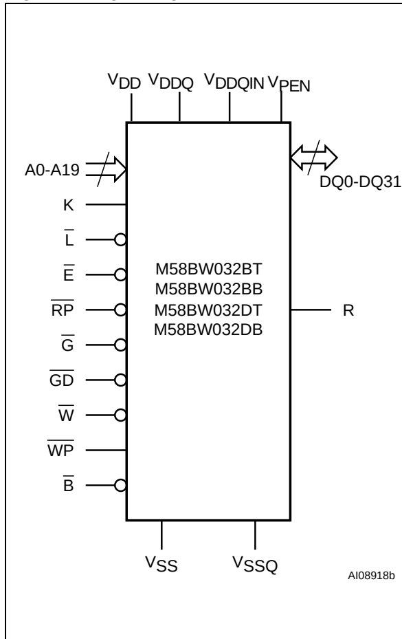
Figure 2. Logic Diagram
