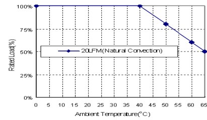
Low Voltage Wattage Derating Curve
