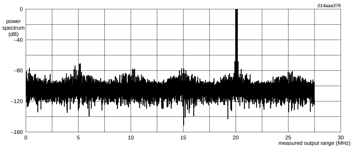
Fig 10. Two-tone; f_1 = 20 MHz; f_2 = 20.1 MHz; f_{clk} = 55 MHz.
