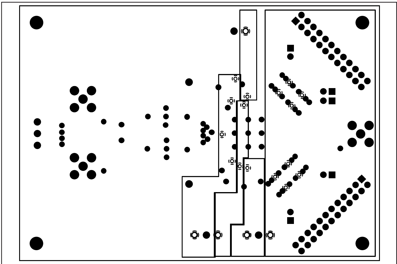
FIGURE 4. Power Plane.
