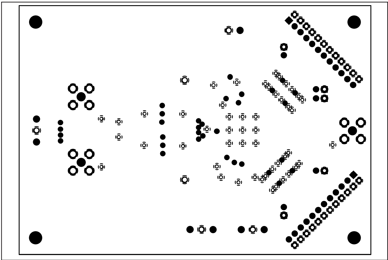
FIGURE 3. Ground Plane.
