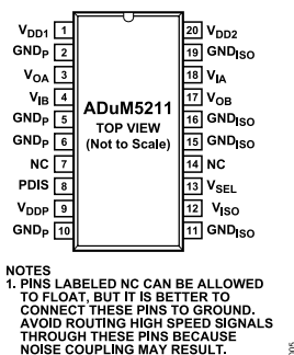
Figure 4. ADuM5211 Pin Configuration
