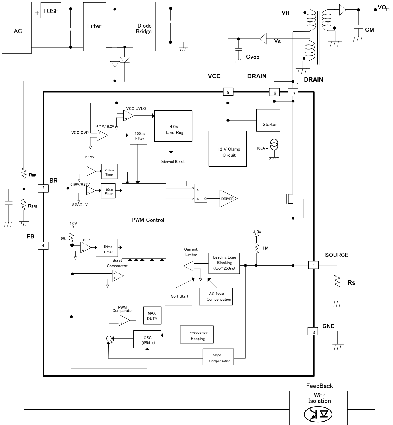
Figure 3. Block Diagram
