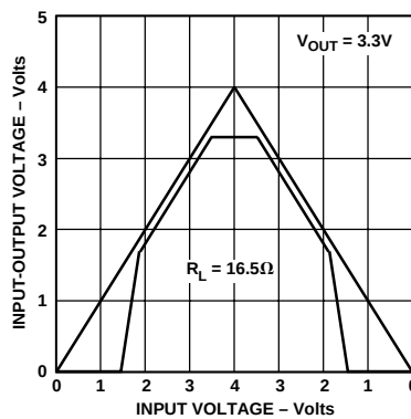
Figure 9. Power-Up/Power-Down
