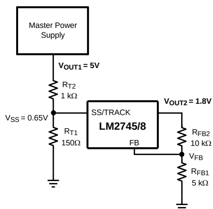
Figure 19. Tracking Circuit
