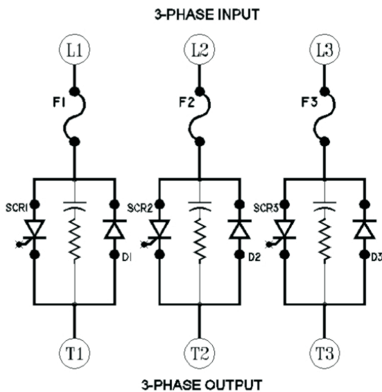
POWER CIRCUIT SCHEMATIC
