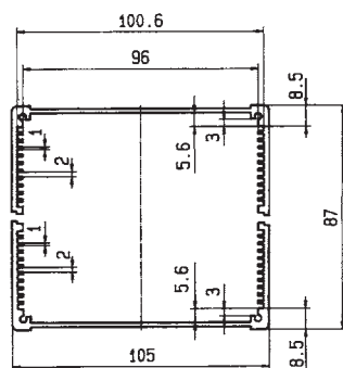
Enclosure Profiles
