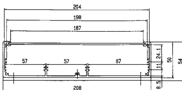
Enclosure Profile
