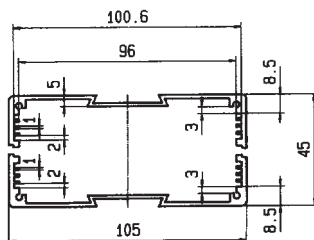
Enclosure Profiles
