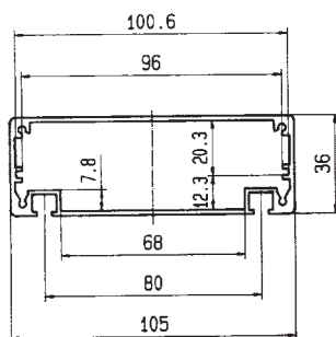
Enclosure Profile
