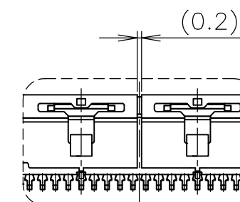
DETAIL C 180P~240P ONLY
