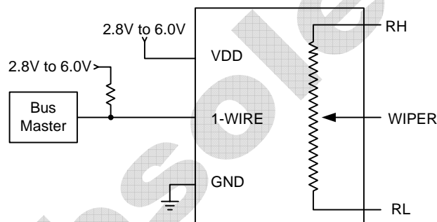
Figure 5. Potentiometer Configuration
