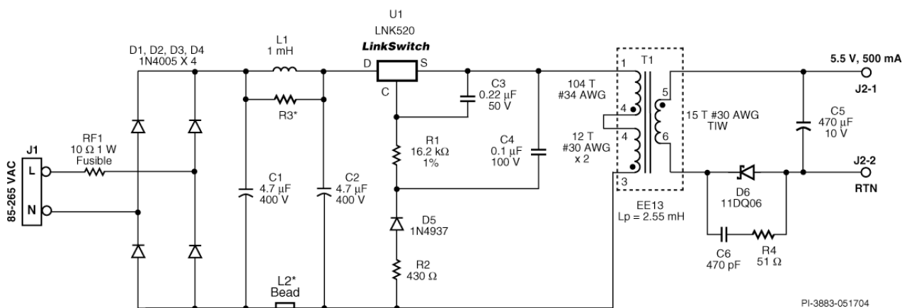
Figure 30 – Modified EP-16: Low Cost, 2.75 W Cell Phone Charger Using the LNK520P.
