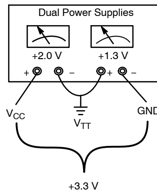
Figure 3. “Split” Power Supply Connections
