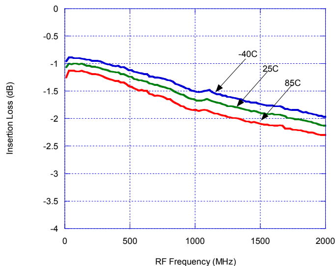
Figure 6. Insertion Loss ( Z_0 = 75\ \Omega )
