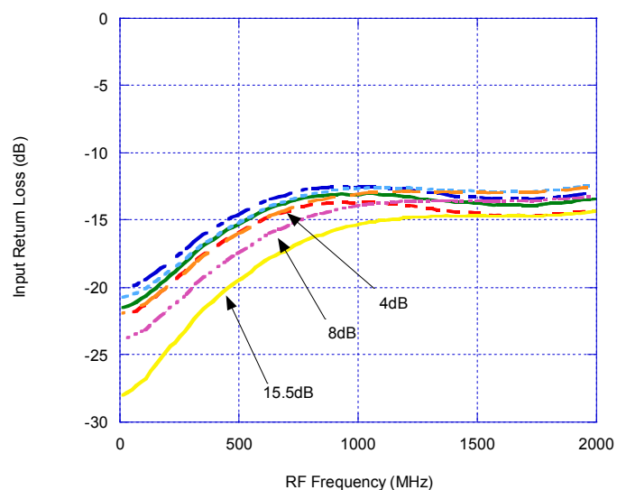
Figure 8. Input Return Loss at Major Attenuation Steps ( Z_0 = 75\ \Omega )
