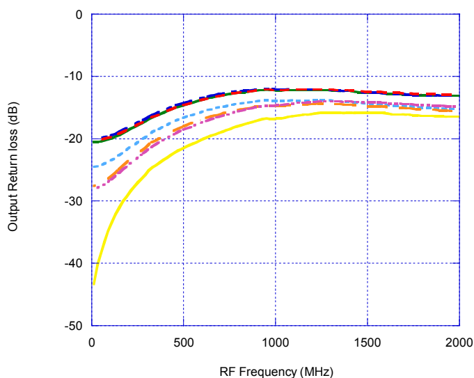
Figure 9. Output Return Loss at Major Attenuation Steps ( Z_0 = 75\ \Omega )
