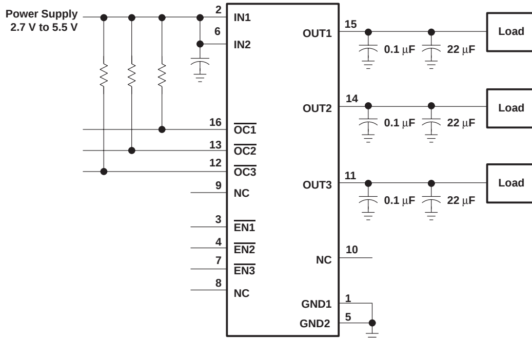
Figure 29. Typical Application
