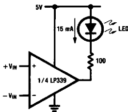
LED Driver
