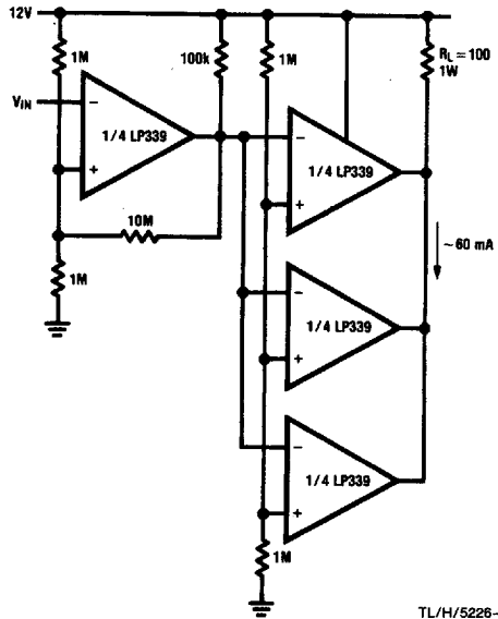
Comparator With 60 mA Sink Capability
