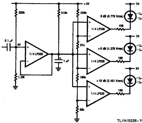
LED Driver
