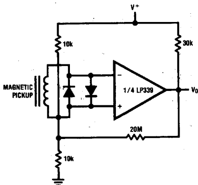
Transducer Amplifier
