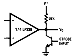
Output Strobing
