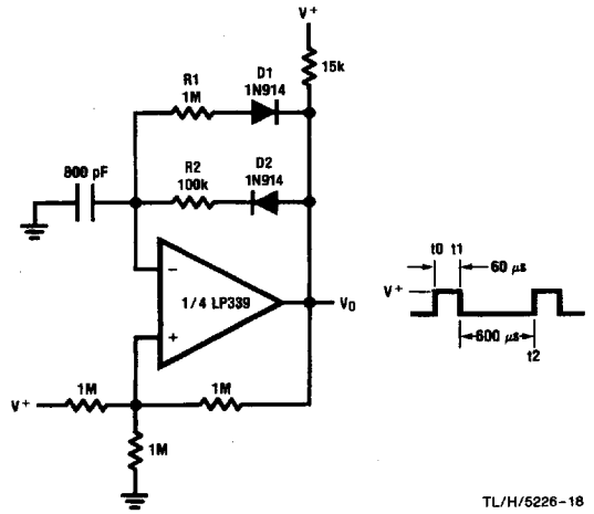
Pulse Generator
