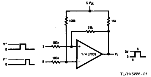
Bi-Stable Multivibrator
