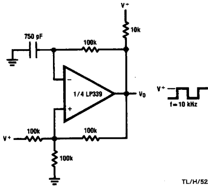
Squarewave Oscillator
