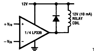
Relay Driver
