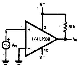
Split-Supply Applications Zero Crossing Detector
