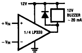
Buzzer Driver
