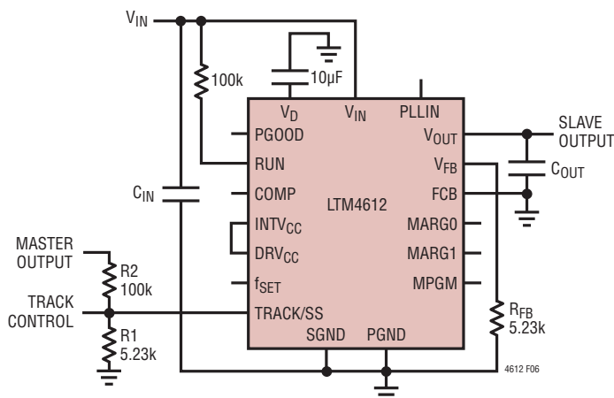
Figure 6. Coincident Tracking
