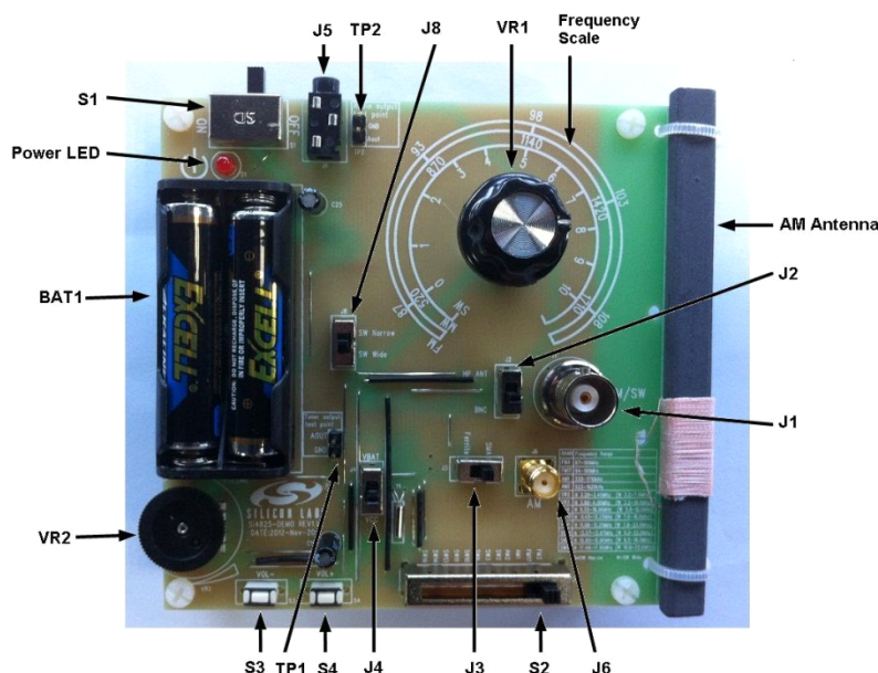
Figure 1. Si4825-DEMO Board Top Side
