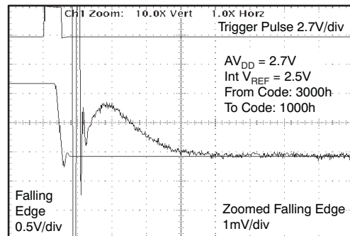
Time (2µs/div)
