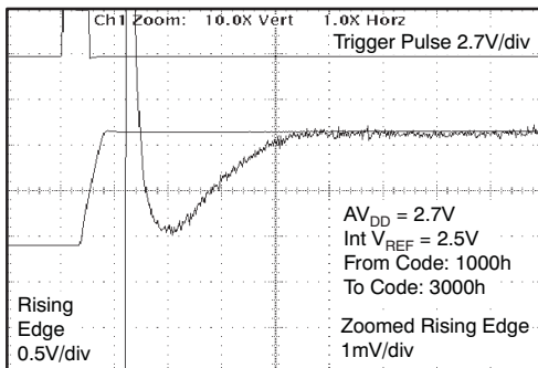
Time (2µs/div)
