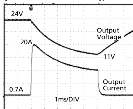
Fig. 25-2 Peak load 20A for 5ms, typ.
