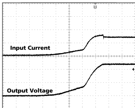
Fig. 6-2 Soft-start behavior
