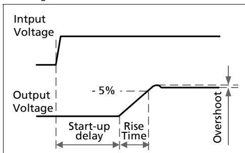
Fig. 5-3 Turn-on behavior, definitions
