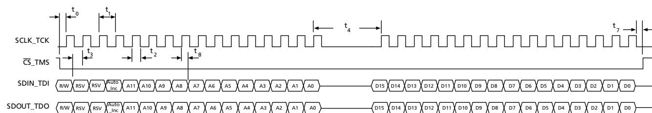
Figure 4-24: Write Mode
