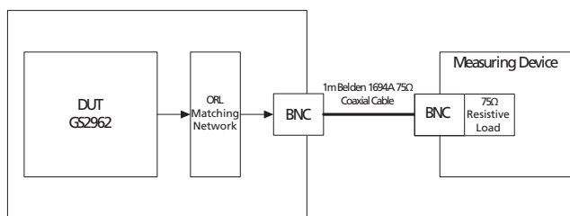
Figure 4-20: ORL Matching Network, BNC and Coaxial Cable Connection
