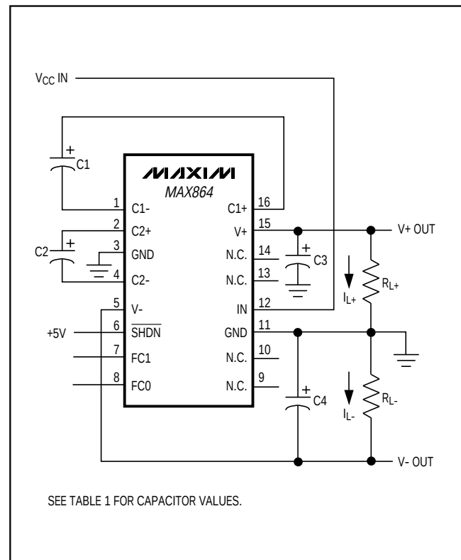
Figure 1. Test Circuit
