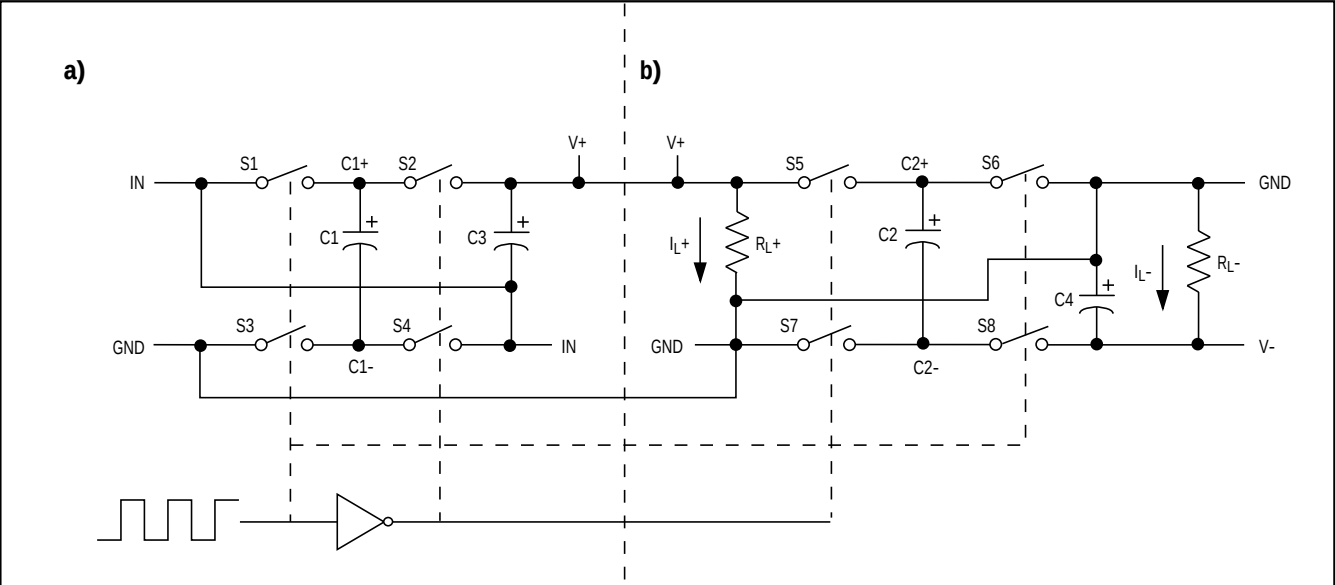
Figure 2. Idealized Voltage Quadrupler: a) Positive Charge Pump; b) Negative Charge Pump
