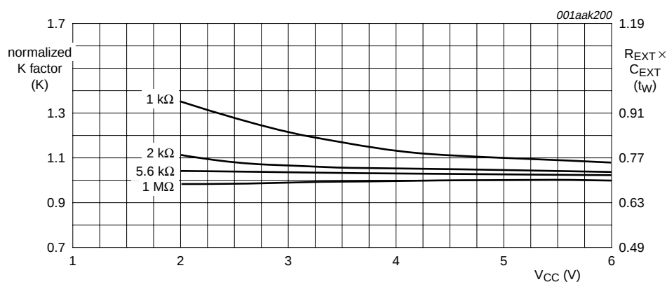
Fig 15. Typical pulse width accuracy versus power supply
