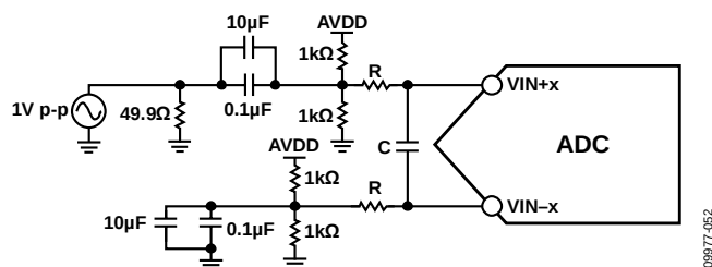
Figure 48. Single-Ended Input Configuration
