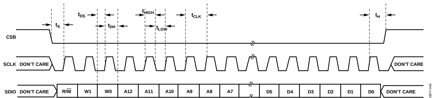
Figure 62. Serial Port Interface Timing Diagram
