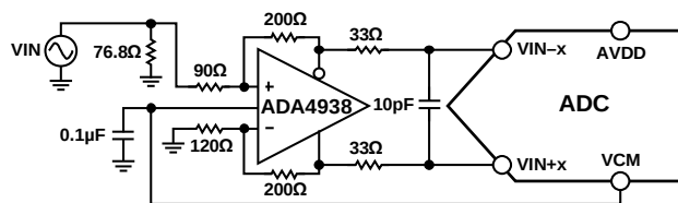
Figure 44. Differential Input Configuration Using the ADA4938-2
