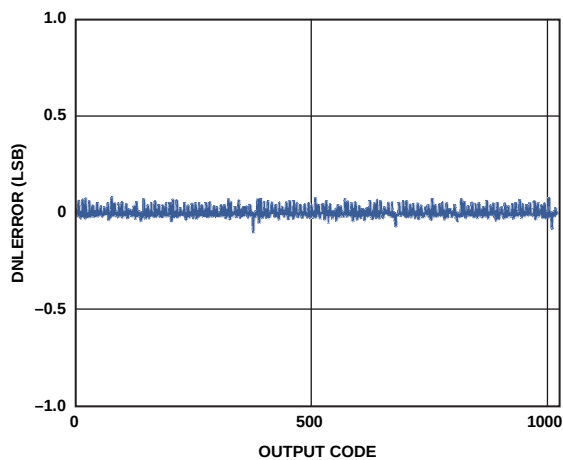
Figure 30. DNL Error with f_{IN} = 9.7 MHz
