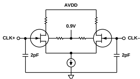
Figure 52. Equivalent Clock Input Circuit
