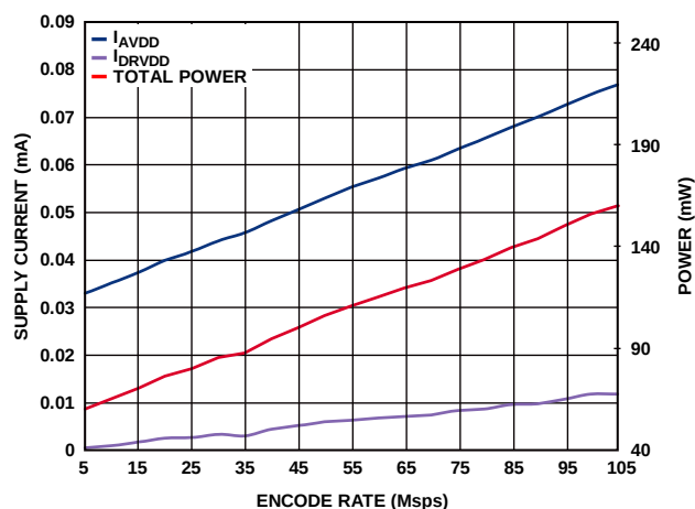
Figure 61. AD9608-105 Power and Current vs. Clock Rate (1.8 V CMOS Output Mode)
