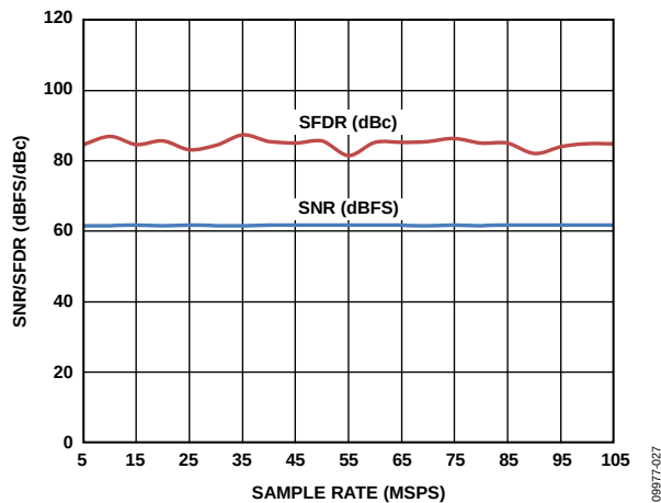
Figure 32. SNR/SFDR vs. Sample Rate with AIN = 70 MHz
