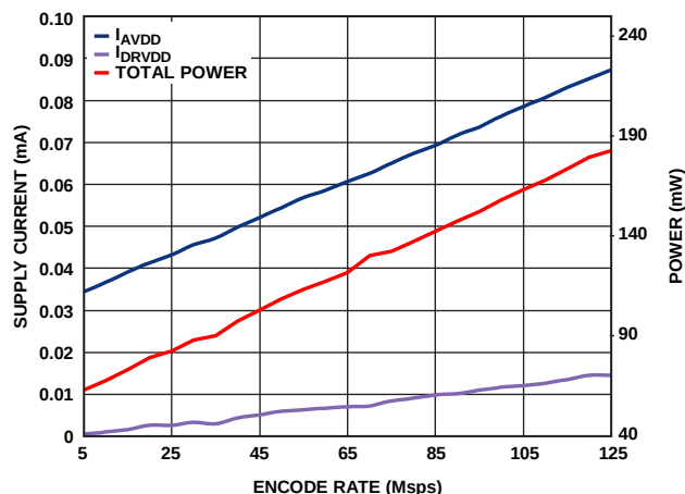
Figure 60. AD9608-125 Power and Current vs. Clock Rate (1.8 V CMOS Output Mode)
