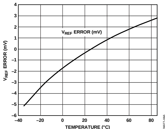
Figure 51. Typical V_{REF} Drift
