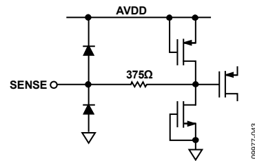
Figure 39. Equivalent SENSE Circuit
