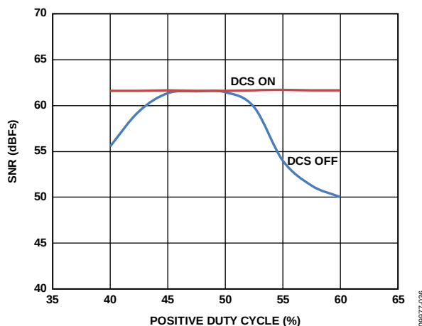
Figure 58. SNR vs. DCS On/Off
