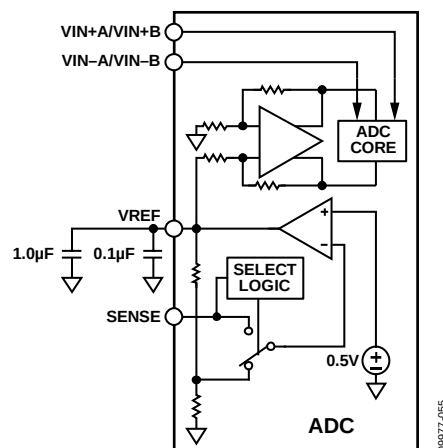
Figure 49. Internal Reference Configuration
