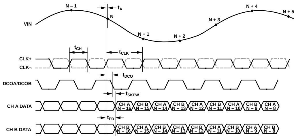
Figure 3. CMOS Interleaved Output Mode Data Output Timing
