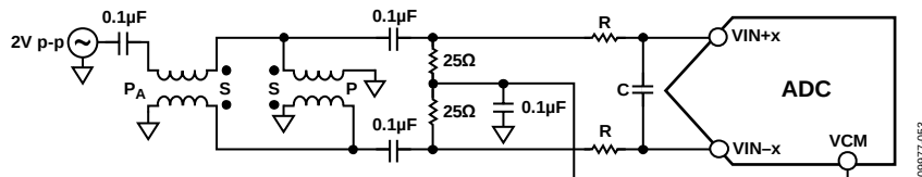
Figure 46. Differential Double Balun Input Configuration
