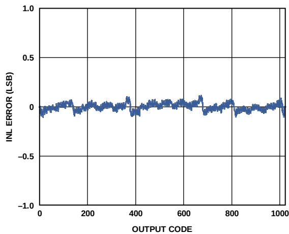
Figure 33. INL Error with f_{IN} = 9.7 MHz
