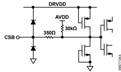
Figure 40. Equivalent CSB Input Circuit
