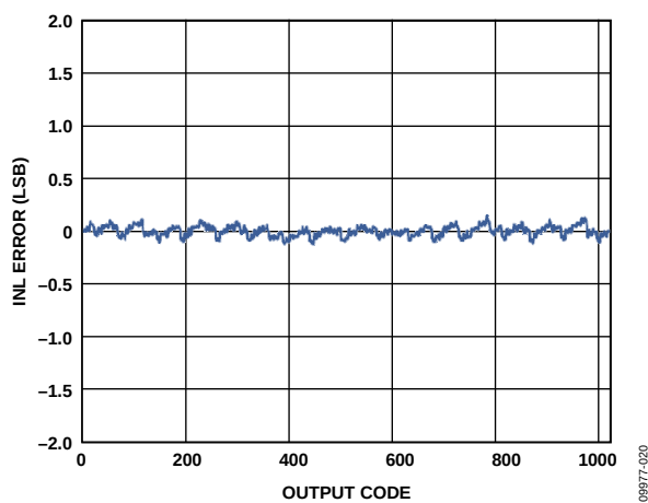
Figure 22. INL Error with f_{IN} = 9.7 MHz
