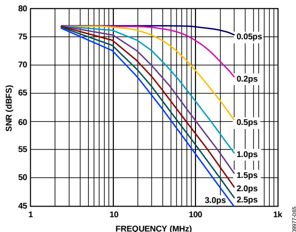
Figure 59. SNR vs. Input Frequency and Jitter
