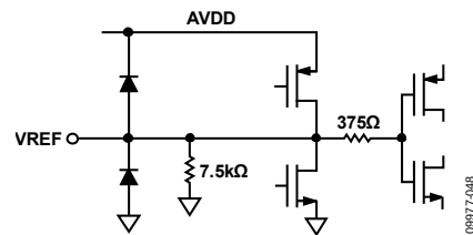
Figure 41. Equivalent VREF Circuit
