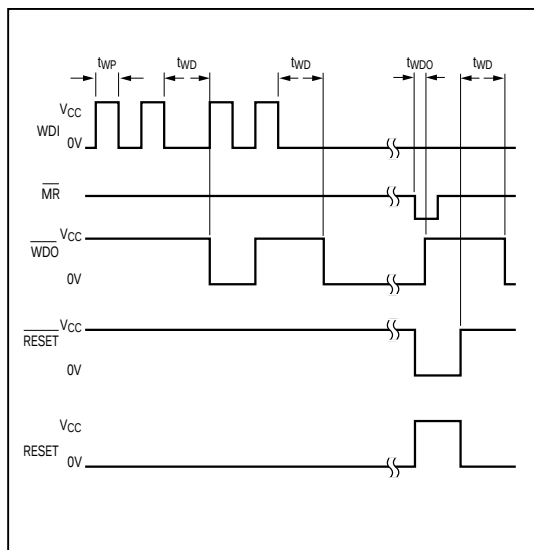
Figure 8. MAX815 Watchdog Timing
