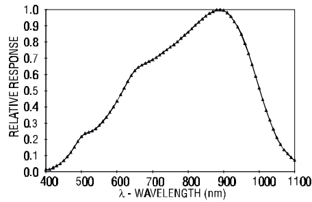
Fig. 6 Spectral Responsivity
