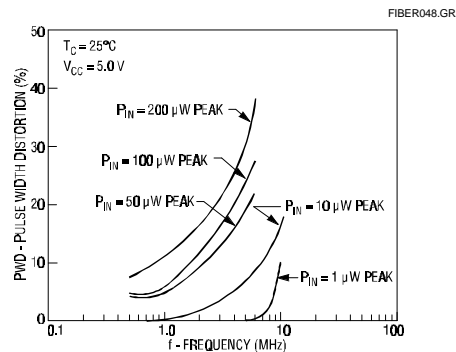
Fig. 2 Pulse Width Distortion vs Frequency
