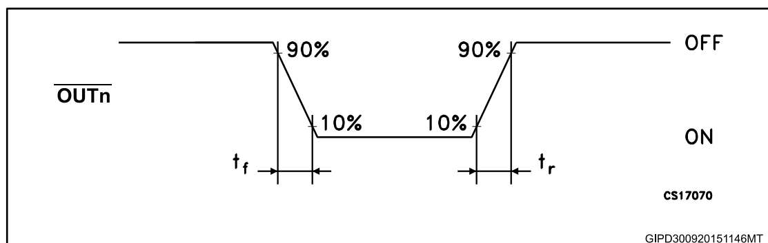
Figure 10: Outputs
