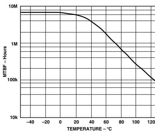
Figure 10. AD2S80A MTBF Curve
