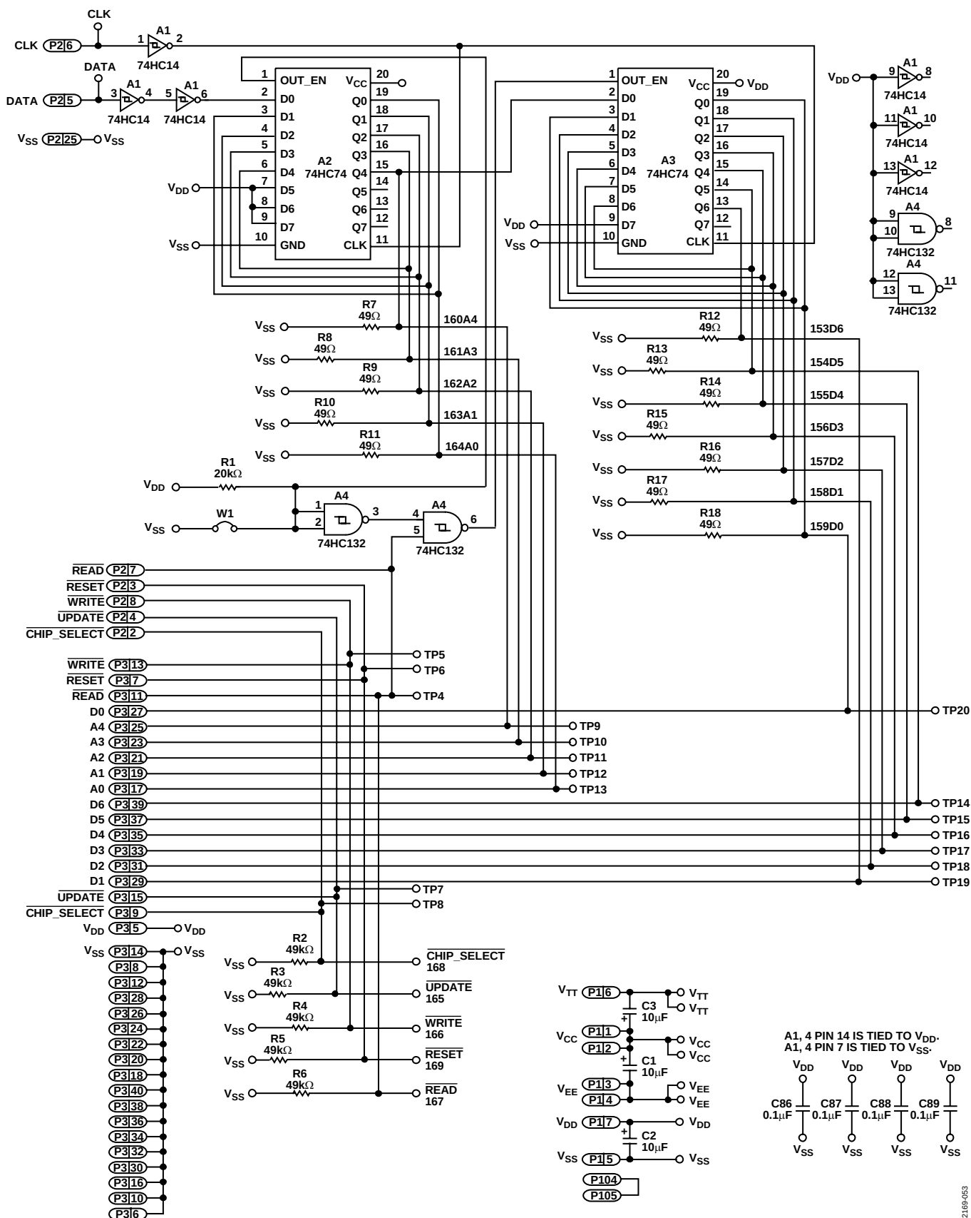
Figure 53. Evaluation Board Logic Controls
