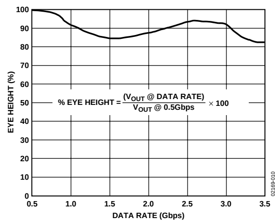
Figure 10. Eye Height vs. Data Rate, PRBS 23
