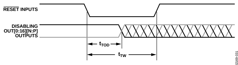
Figure 31. Asynchronous Reset
