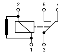
Change Over with Resistor (B)
