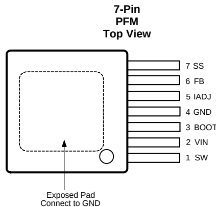
Pin Functions
