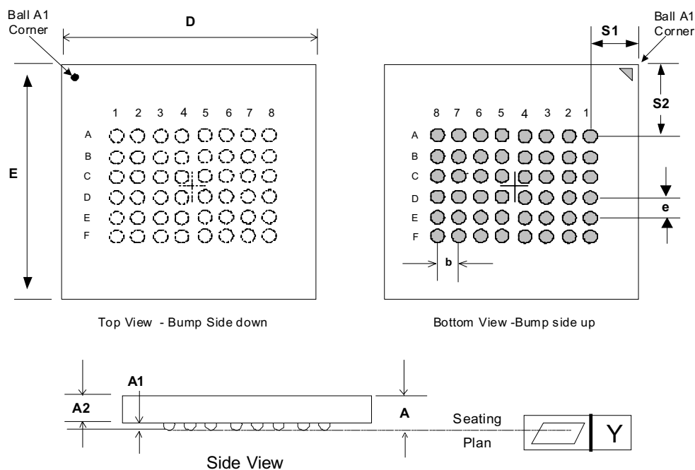
Figure 16. Very Fine Pitch BGA (VF BGA) Package Drawing and Dimensions
