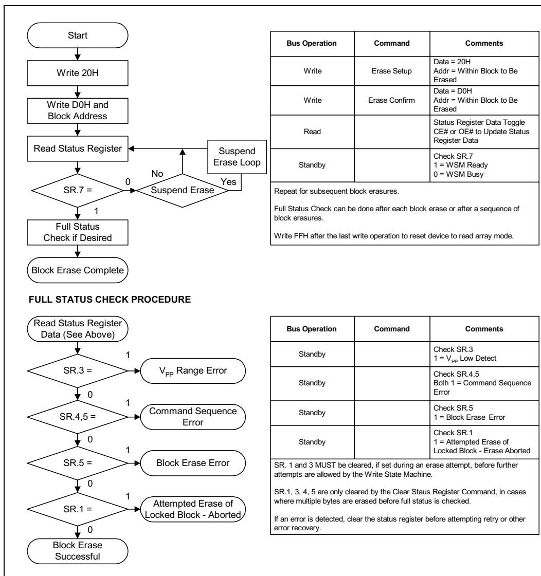
Figure 14. Block Erase Flowchart
