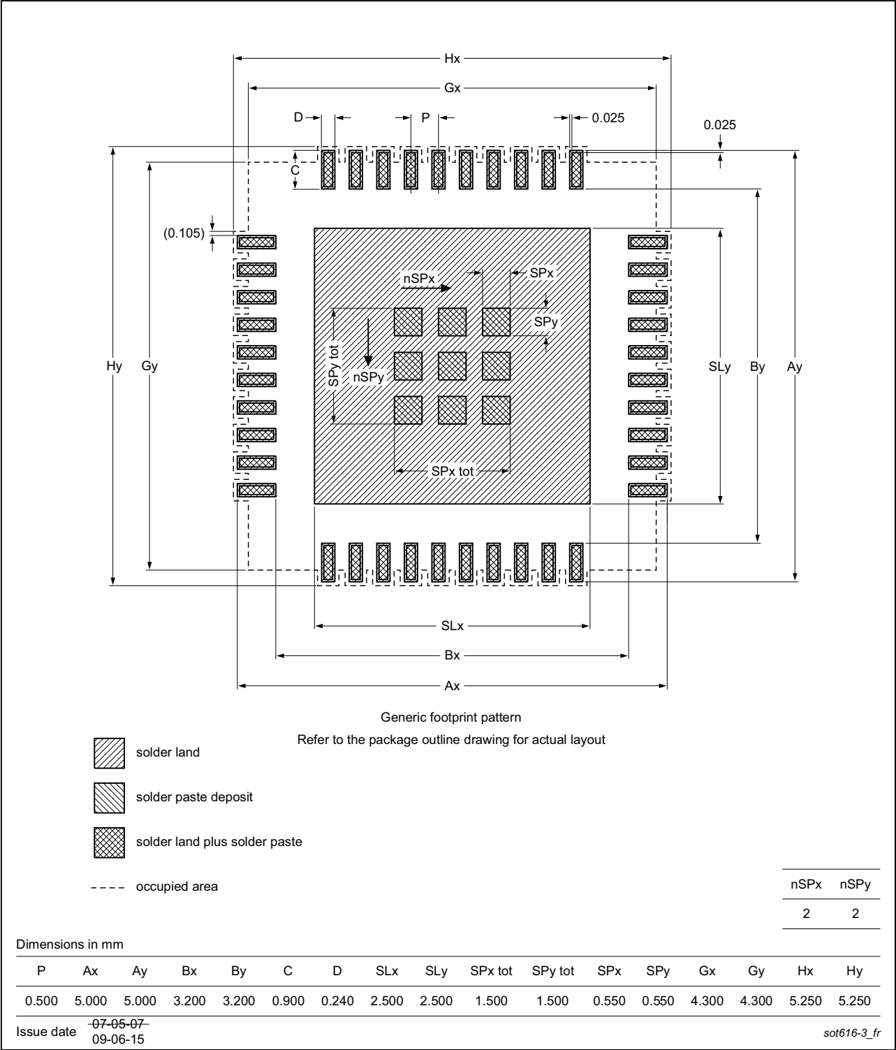
Footprint information for reflow soldering of HVQFN24 package SOT616-3
