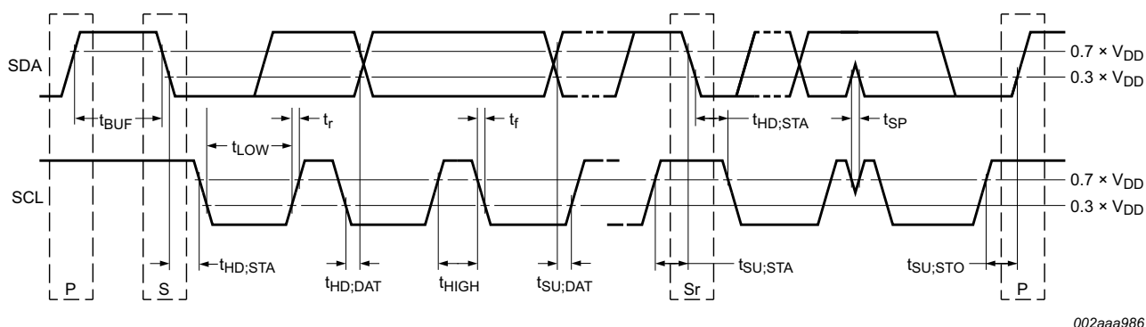
Fig 19. Definition of timing
