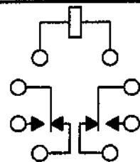
TERMINAL VIEW
