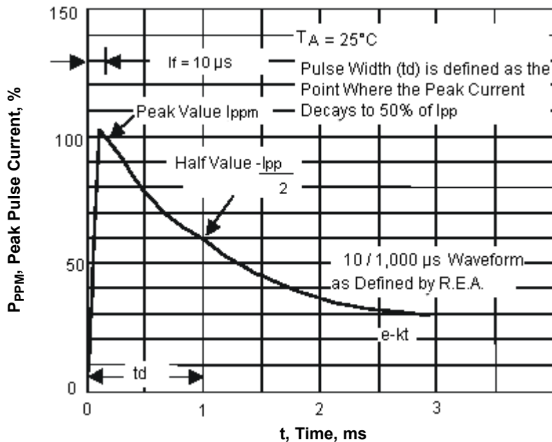
Fig. 3-Pulse Waveform
