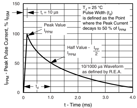
Fig. 2 - 10/1000 \mu\text{s} Pulse Waveform
