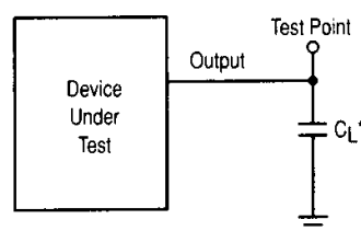
Figure 6. Test Circuit
