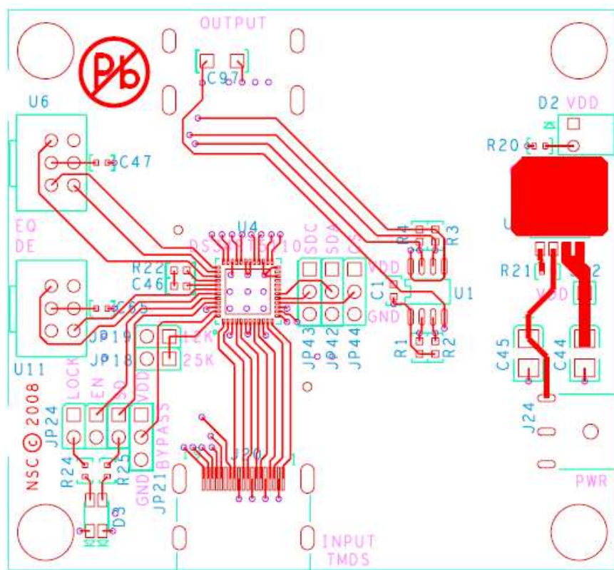
Figure 3. Top Layer
