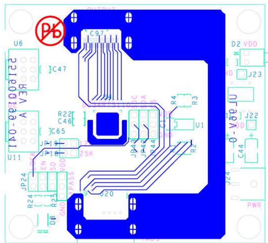
Figure 4. Bottom Layer
