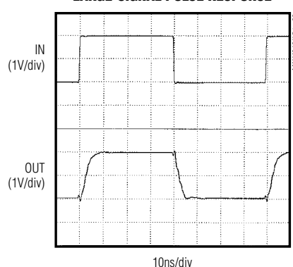
MAX4310 LARGE-SIGNAL PULSE RESPONSE
