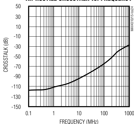
MAX4310/MAX4313 ALL-HOSTILE CROSSTALK vs. FREQUENCY
