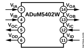
Figure 3. ADuM5402W
