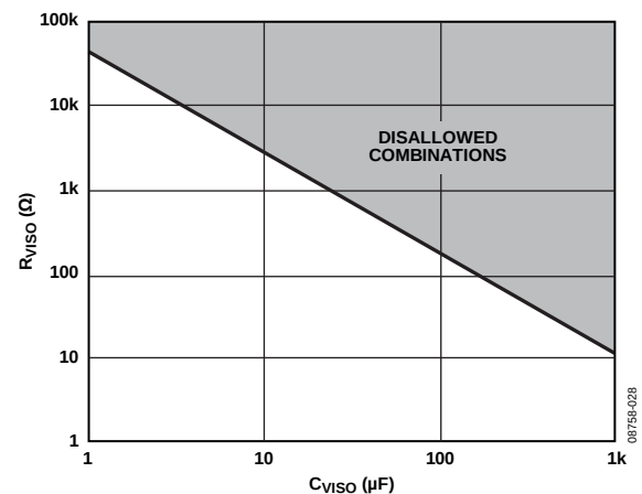
Figure 31. Maximum Capacitive Load for Proper Restart
