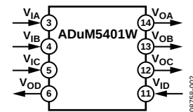
Figure 2. ADuM5401W
