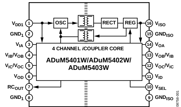
Figure 1. ADuM5401W/ADuM5402W/ADuM5403W Block Diagram
