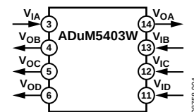
Figure 4. ADuM5403W
