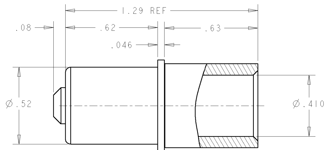
SECTION Z-Z
