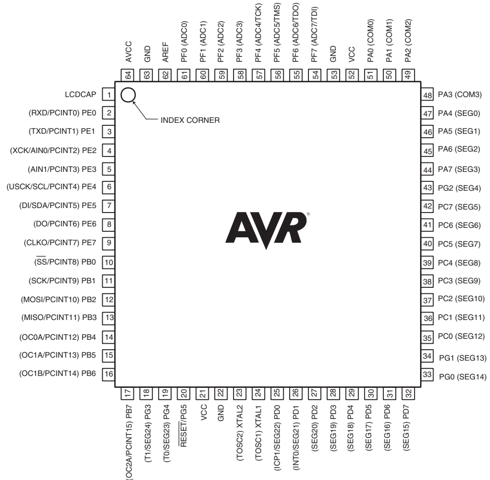
Figure 1-1. Pinout ATmega169P
