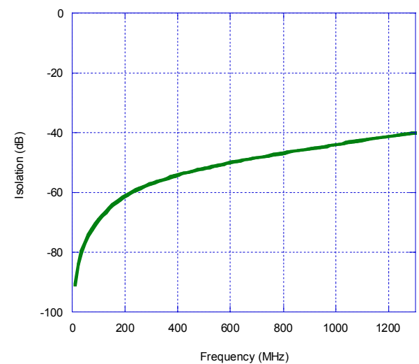
Figure 7. Isolation – RFC to RF1
