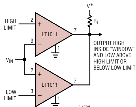
Window Detector
