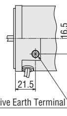
Detail Drawing of Protective Earth Terminal
