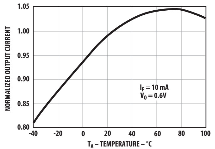
Figure 2 Normalized Output Current vs. Temperature
