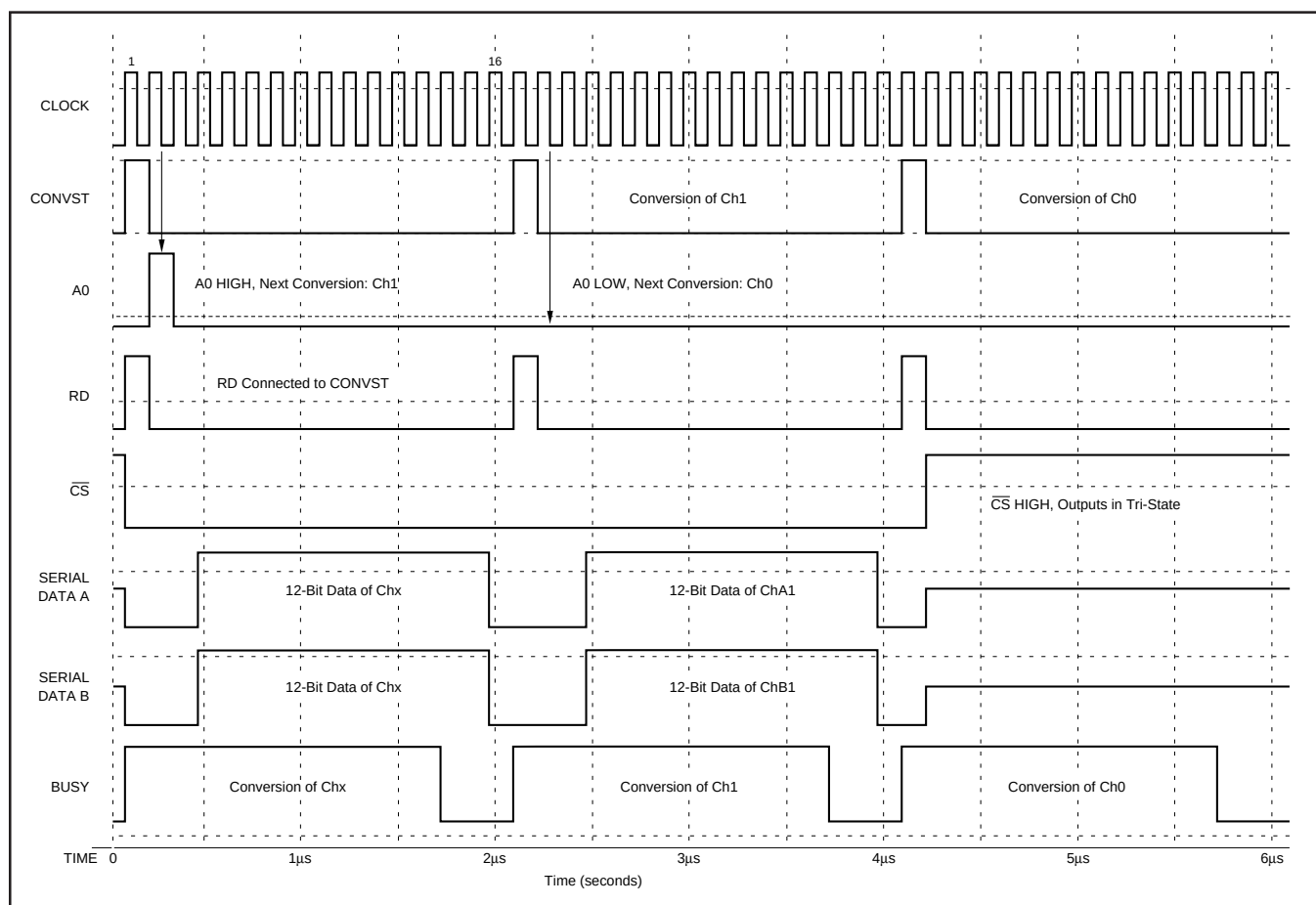
FIGURE 10. Mode I, Timing Diagram for M0 = 0 and M1 = 0.
