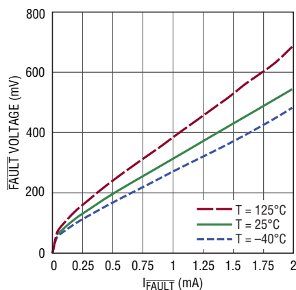
\overline{\text{FAULT}} Output Voltage
